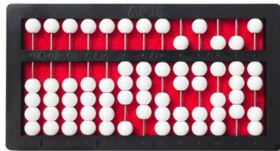
A Cranmer abacus has 5 beads on each rod. The red felt backing prevents the beads from moving once they have been set in position. This abacus is set to read 34,172,692.
